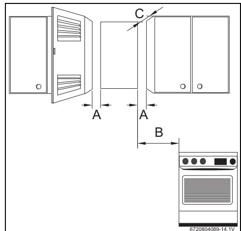
Fig. 19 Distances minimales
