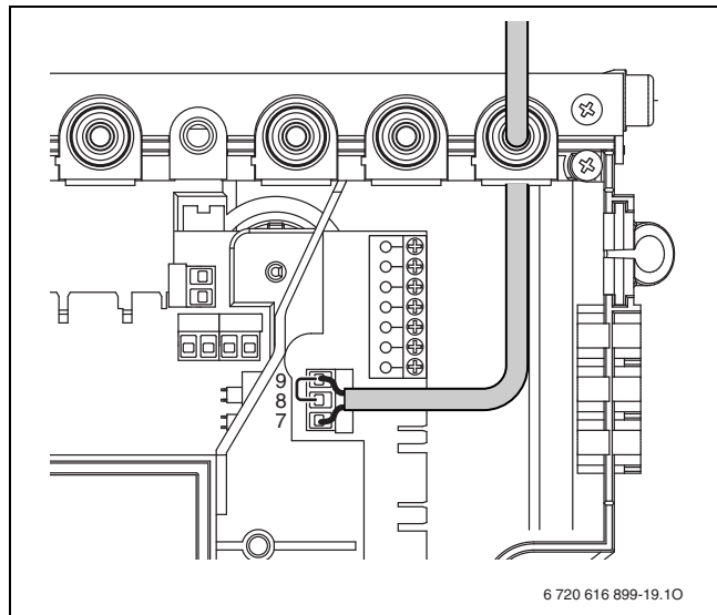
Fig. 48 Raccord thermostat
