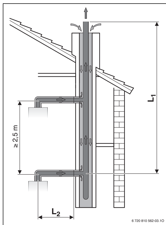
Fig. 27 Configuration C 43p
