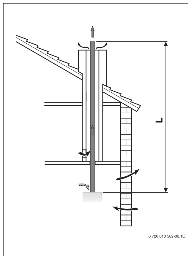
Fig. 18 Configuration B 23p verticale
